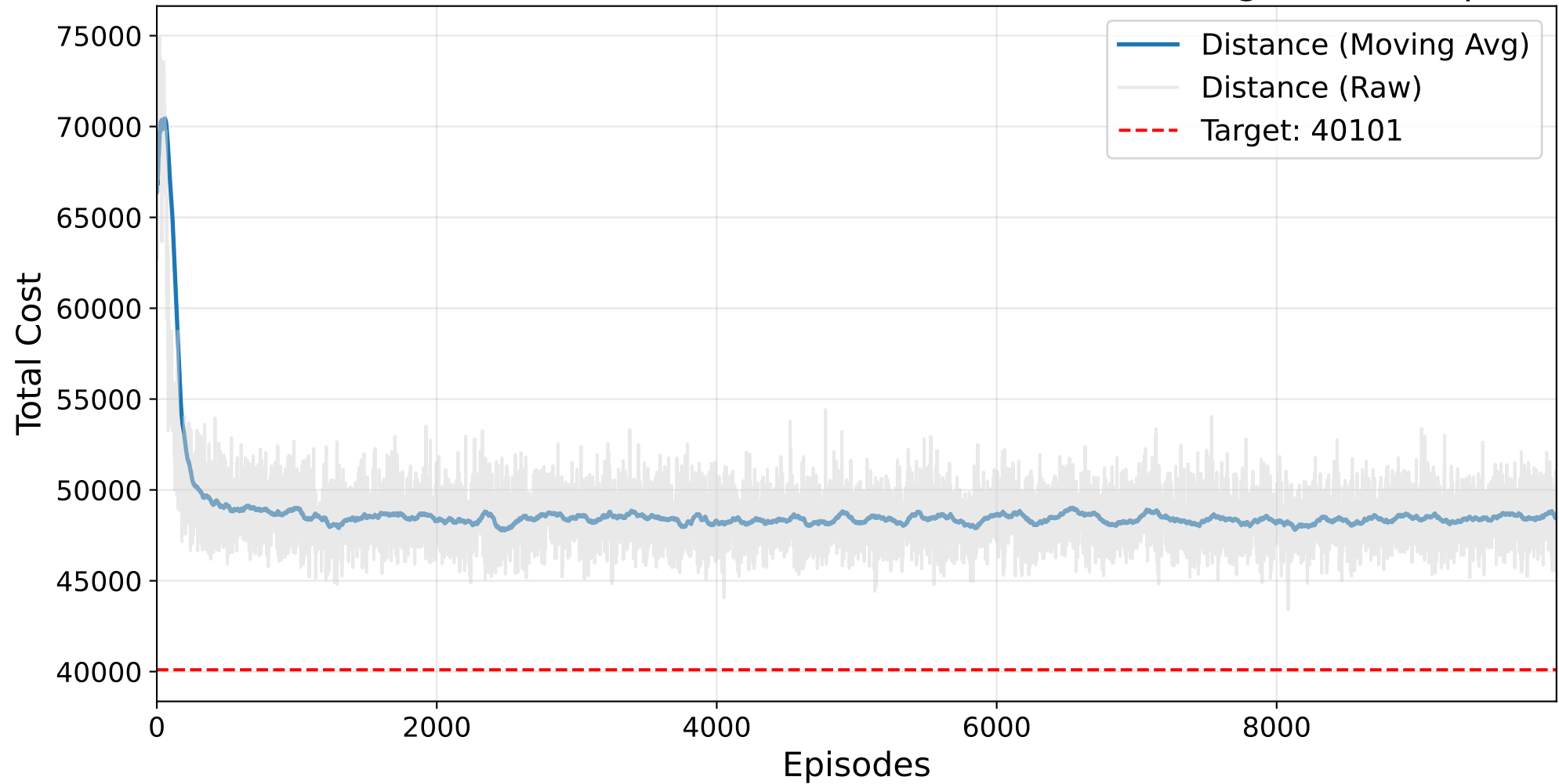
Final GAUSSIAN PROCESS Masked AutoRL-SOP Training - ft70.2.sop
